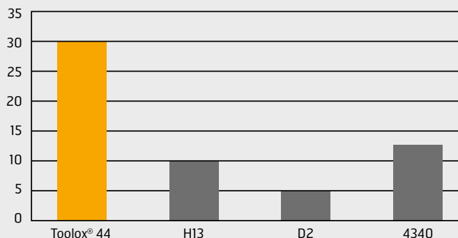
Impact toughness, Charpy-V (J) at 20°C
